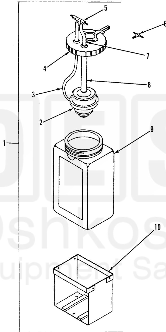
DETAIL A
